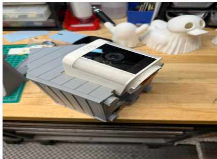
Step 3: Insert camera into housing
