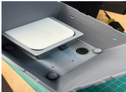
Step 4 (continued): Thumbscrew installed from inside housing
